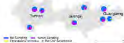
Fig. 9: Concurrent sampling in bats and target human population in communities in Yunnan, Guangxi, and Guangdong provinces. Pie-charts indicate sampling effort (bat sampling = blue, Human questionnaire and sampling = purple, Ethnographic interview = yellow, bat CoV seropositive = red)
